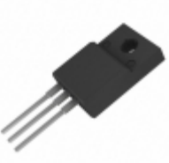
FDPF79N15 Fairchild/ON Semiconductor MOSFET N-CH 150V 79A TO-220F
