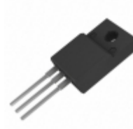
FDPF770N15A Fairchild/ON Semiconductor MOSFET N-CH 150V 10A TO-220F
