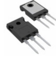
IRG4PC40WPBF Infineon Technologies IGBT 600V 40A 160W TO247AC
